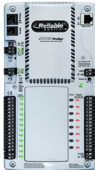
1 MACH-ProSys™ controller
